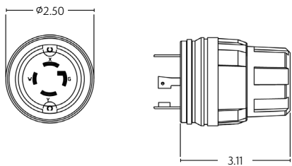
20/30-Amp Locking 4 & 5p, 4 & 5w
