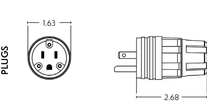
10/15/20-Amp Straight, 15-Amp Locking
